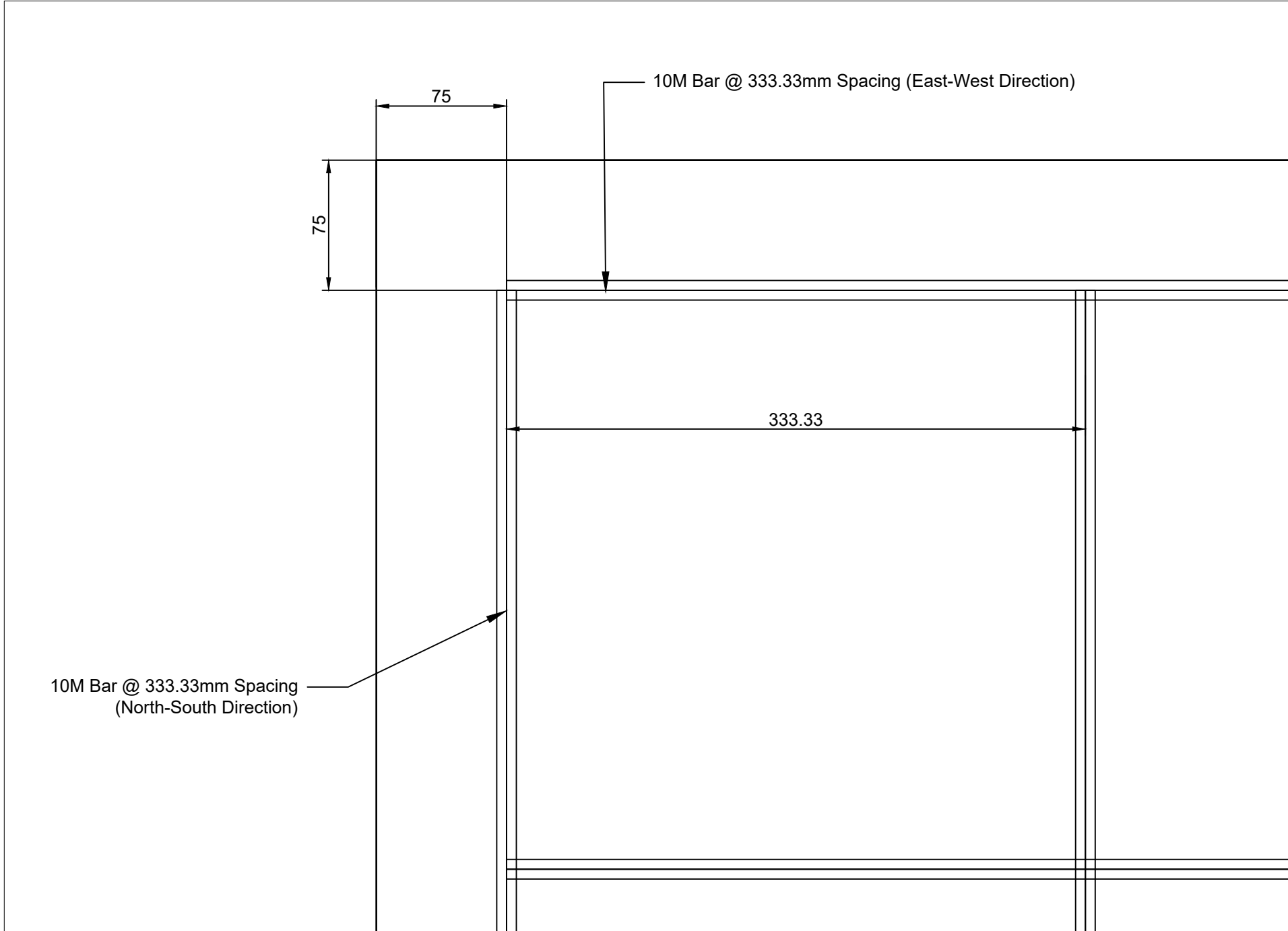
Plan View (Detail Drawing)
